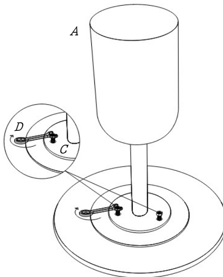
BOLT (7 X 12 MM 3 PCS, EXTRA 2 PCS)
